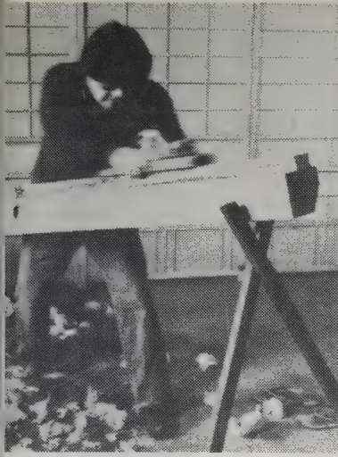
Shokunin [artisans] plane long materials using a pull stroke down an angled planing beam. Speed, a small blade angle, and holding the blade on a skew to the wood help the plane leave a smooth, highly polished surface.
